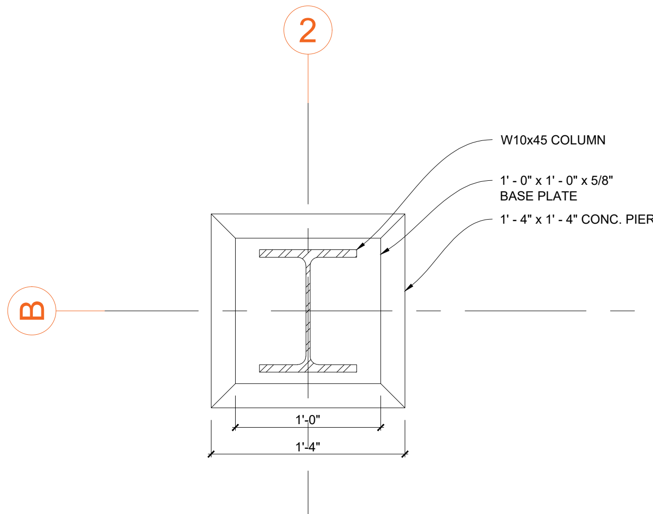
2 COLUMN B2 DETAIL SCALE: 1 - 1/2" = 1' - 0"
